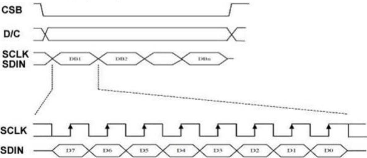
Figure 6-4-2: Write procedure in 4-wire SPI mode
